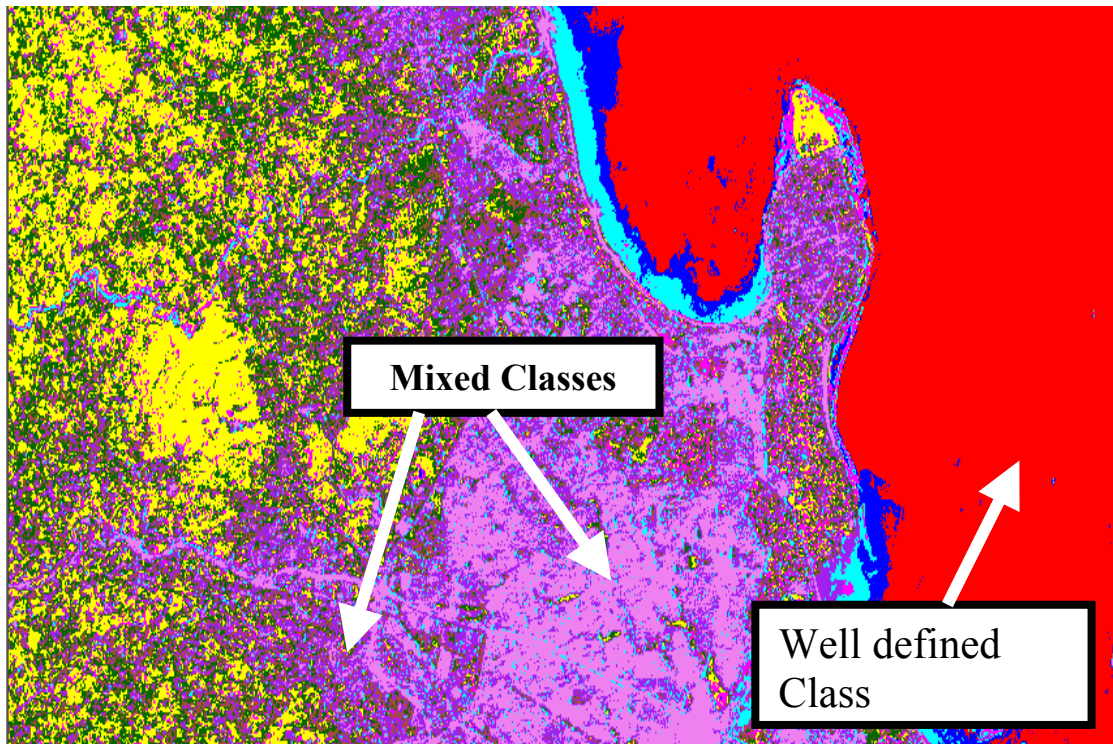
Fig. 3-8: Clustered Image
