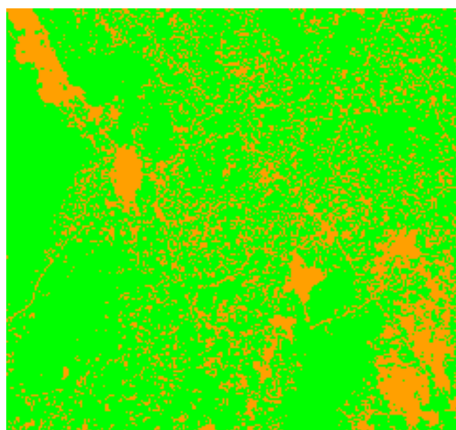
Fig. 6-23:1998, Interpreted Image
