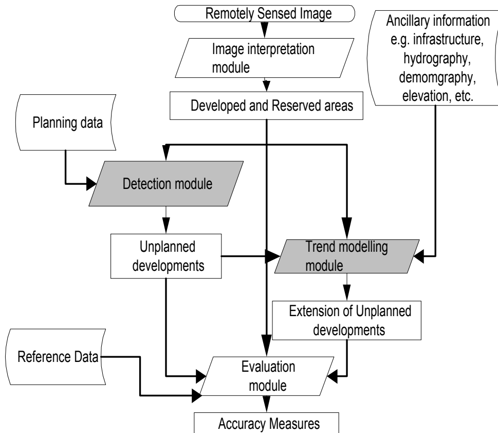
Fig. 4-1: The Detection and Trend Modelling Modules
